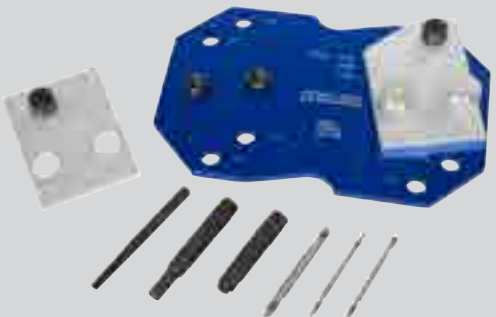
Exhaust Manifold Drill Template Set for Ford 2v & 3v 68500
