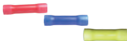
BUTT CONNECTORS - VINYL INSULATED 1700-CS - red, 22-18 AWG 1800-CS - blue, 16-14 AWG 1900-CS - yellow, 12-10 AWG
